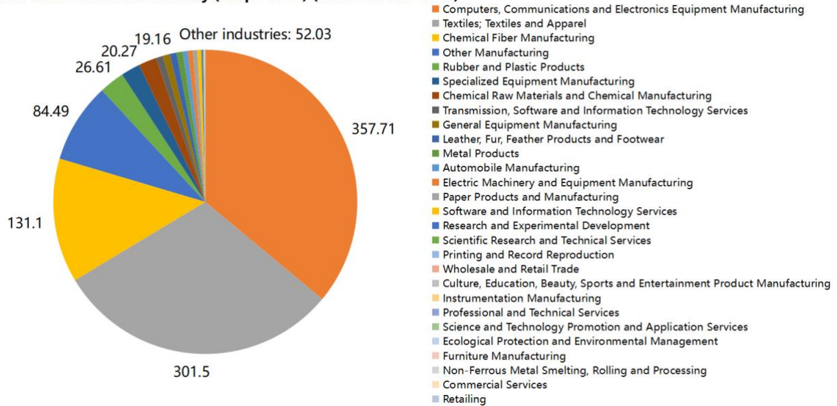
Total emissions of the industry (Scope 1 + 2) (ten thousand CO 2 e)
