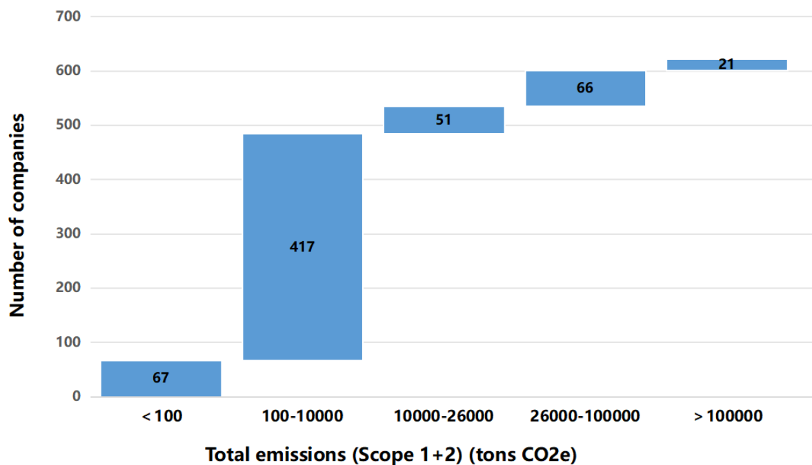
Figure 1 Distribution Range of Enterprise GHG Emissions (Scope 1+2)
